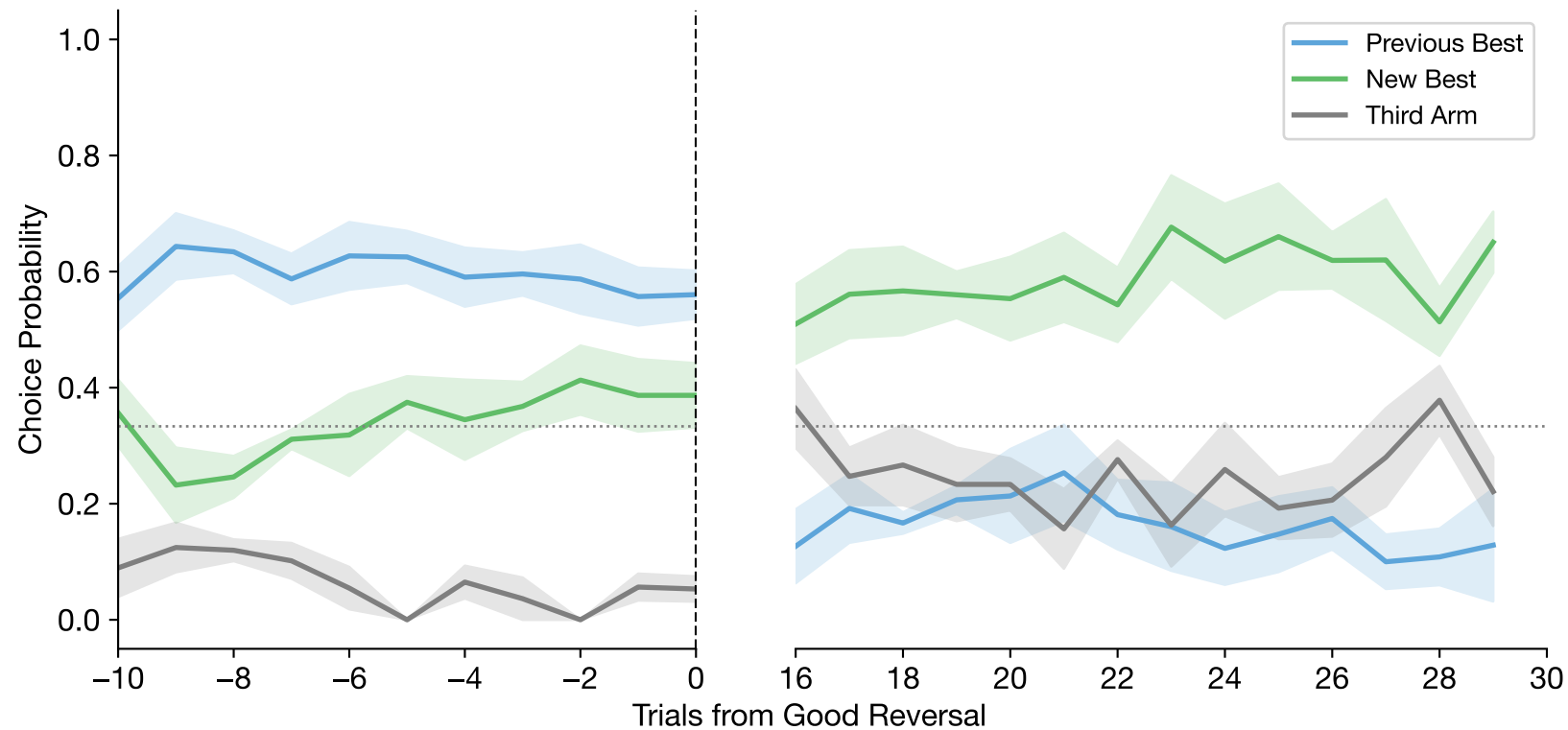
Good Reversal-Aligned Choices (mean \pm se across subjects | n=5 subjects, n=51 reversals) (Skipping first 15 trials post-reversal)
